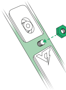
10.1 Place the bottle cage on the baseplate, so that the protruding bolt passes through it and you can install the nut to hold it down.
