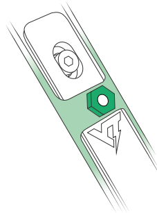
10.2 Tighten the nut with 2 Nm of torque.
