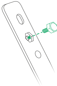
9.3 Push the bolt through the baseplate from the bottom...
